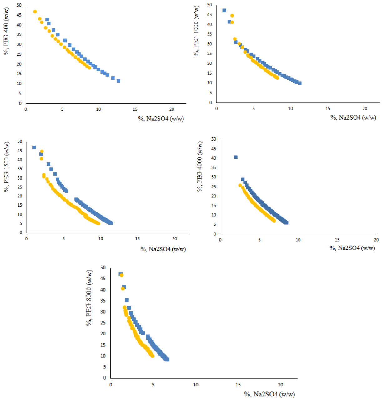
Figure 1. Binodal curves to systems containing PEG + Na 2 SO 4 + H 2 O in absence (■) and presence (●) of 5 wt% KI at 298.15 \pm 1 K and atmosphere pressure.
