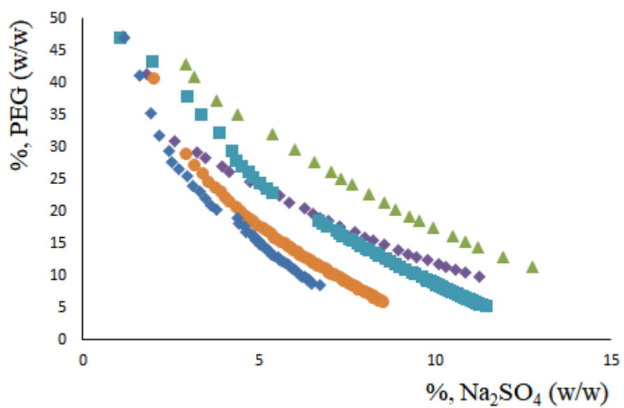
Figure A.2. Binodal curves to systems containing PEG 400 (▲), 1000 (■), 1500 (◆), 4000 (●) and 8000 (◆) g.mol -1 + Na 2 SO 4 at 25 °C and atmospheric pressure
